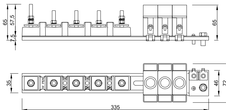
SR 563-14, IP 00
