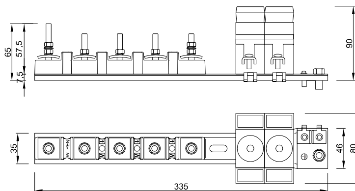
SR 562-25, IP 00
